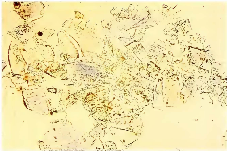
PLATE 6. Photomicrograph of smalt, \times 300 , from Yūgo with a Pipe Standing in the Open Side of a Room and Looking Out , in the style of Miyagawa Chōshun (1682–1752). Japan, Edo period (1615–1868). Hanging scroll; color and ink on paper; 98.6 \times 46.0 cm (F1903.134). In transmitted light, mounted in Canada balsam, \eta=1.53 .
